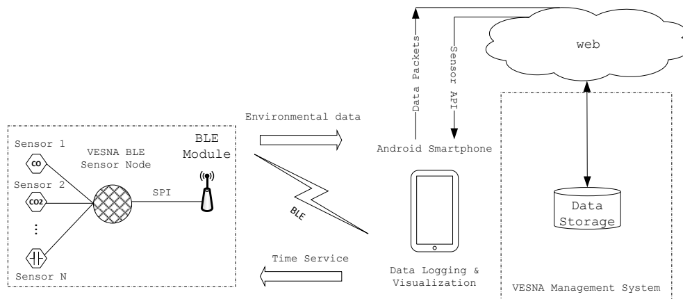
Figure 14-8 VESNA BLE system
