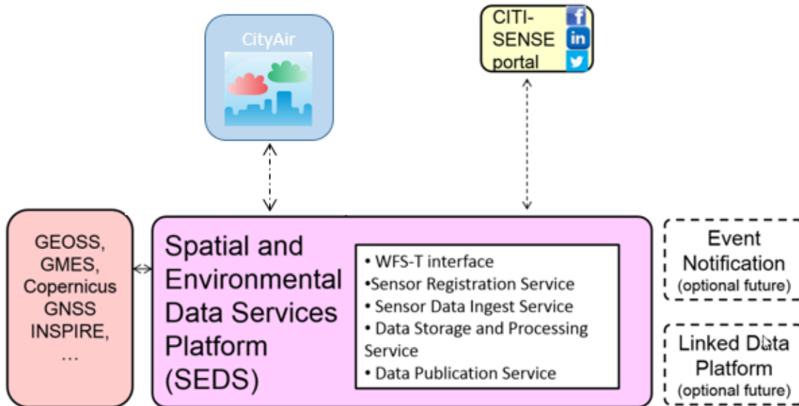
Figure 13-1 Data Flows for the CityAir architecture
