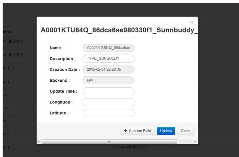
Figure 3-8 Sensor description
