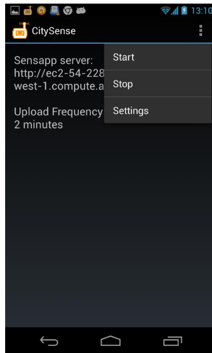
Figure 9-5: Configuration
