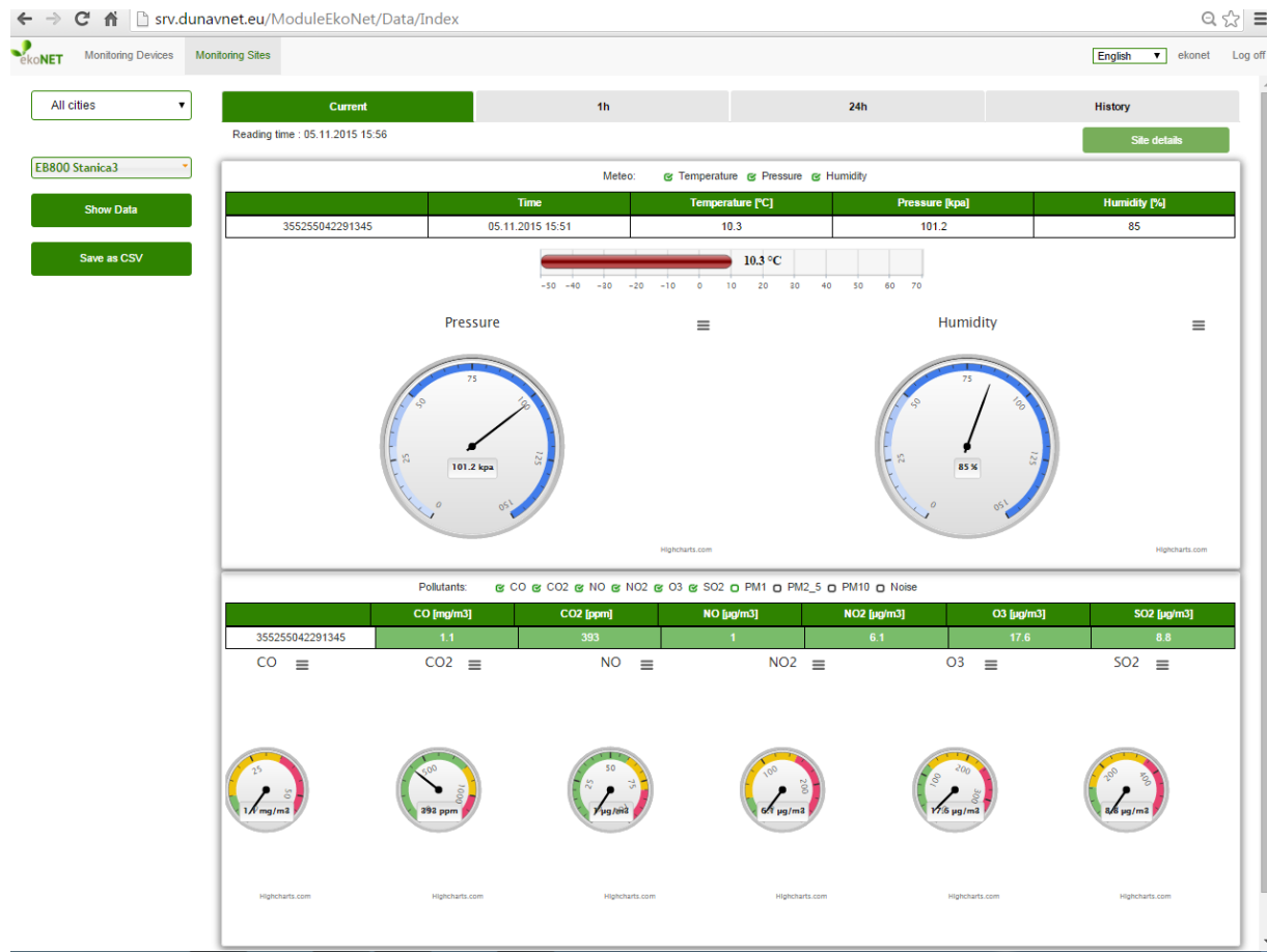
Figure 15-6 Web portal
