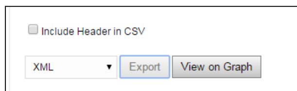
Figure 6-6 Exporting data
