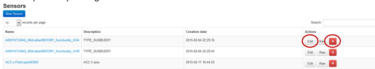
Figure 3-7 Managing sensors
