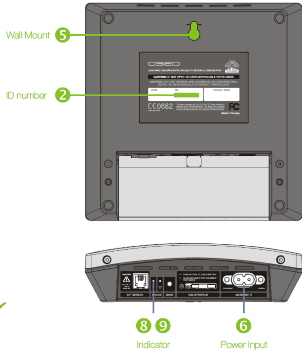
Figure 8-2 OBEO MMA Radon sensor installation process and connectors
