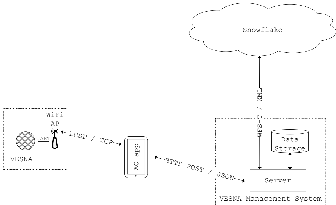
Figure 14-2 VESNA Air Quality Monitoring System Architecture
