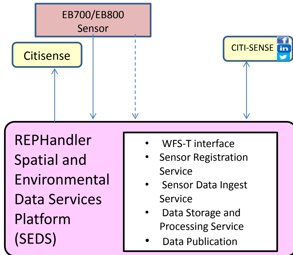
Figure 15-3 Data Flows for the CITI-SENSE DNET architecture
