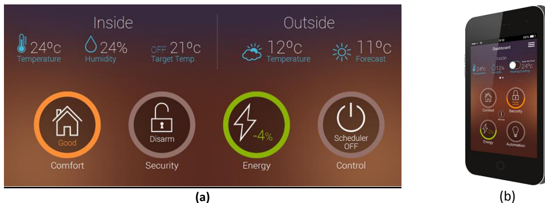
Figure 10-2: enControl™ Dashboard
