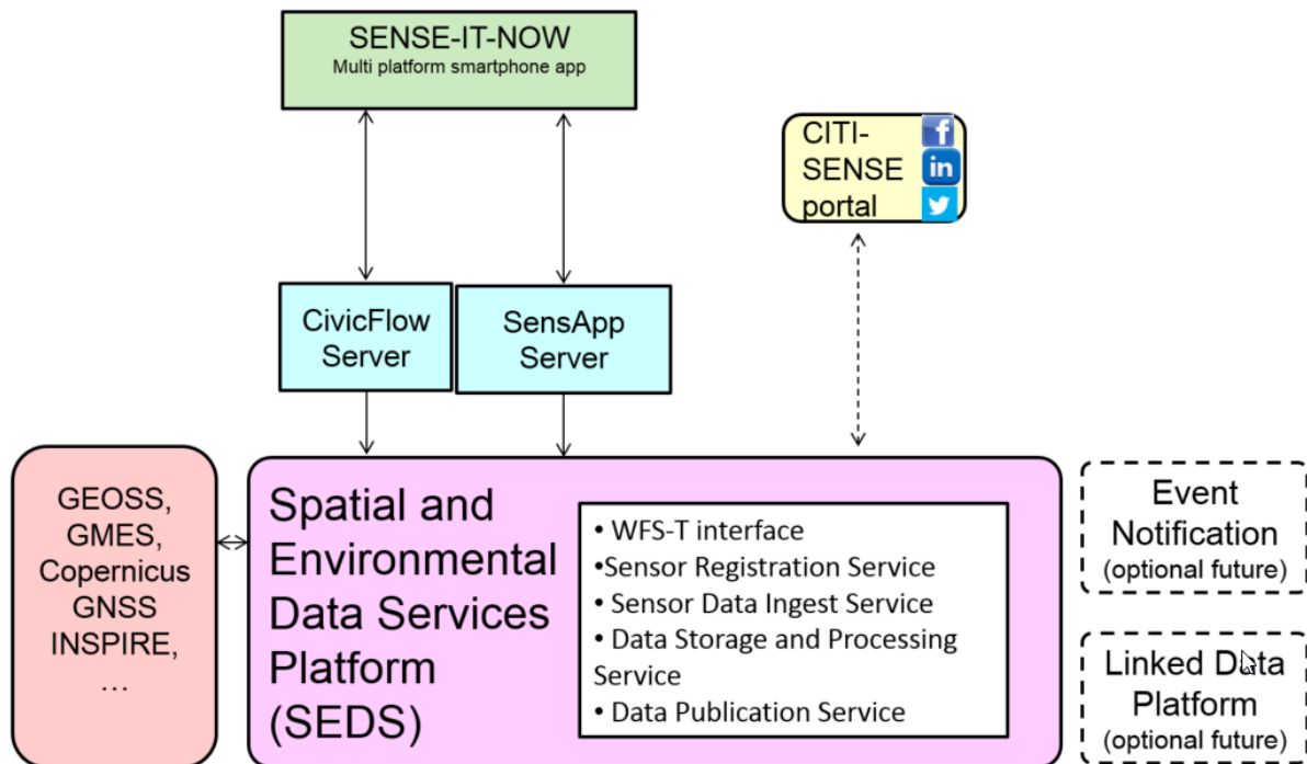
Figure 11-1 Data Flows for the SENSE-IT-NOW architecture
