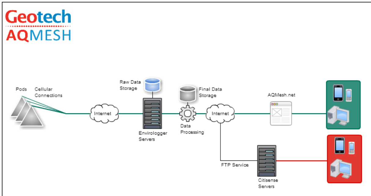
Figure 6-3 AQMesh data flow
